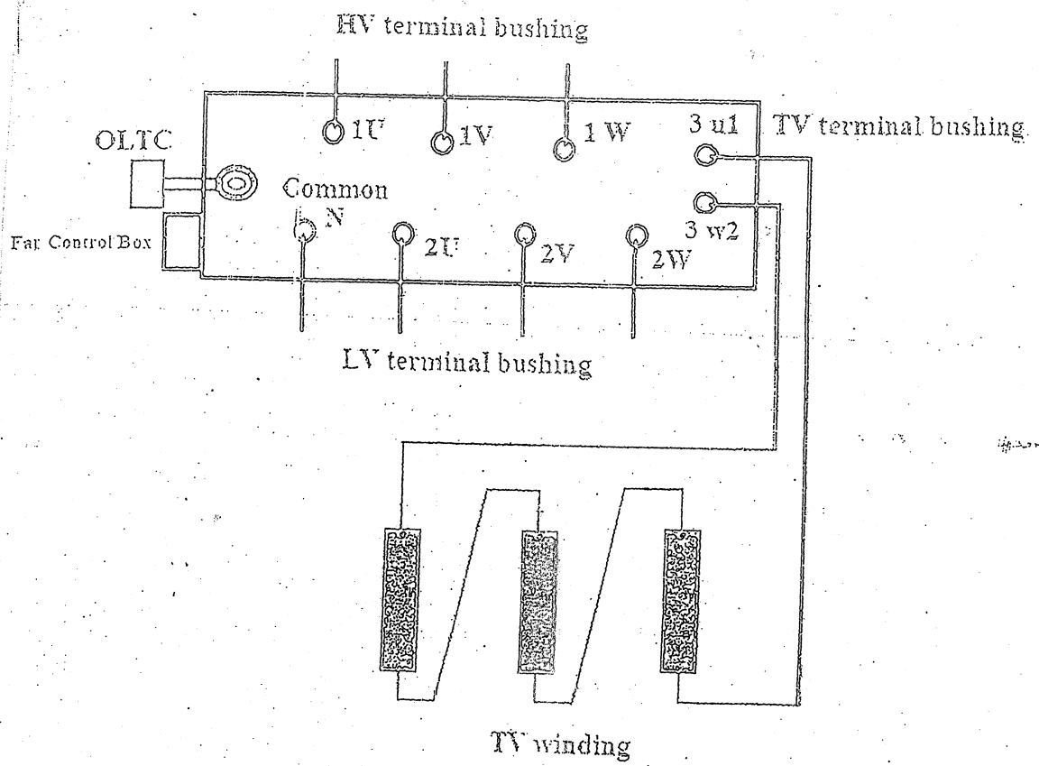
Fig : layout of HV, LV, TV bushing & OLTC
